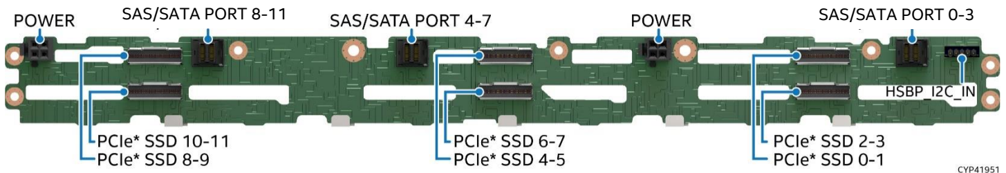
Figure 74. 12 x 2.5" SAS/SATA/NVMe* Hot Swap Backplane – Back Side
