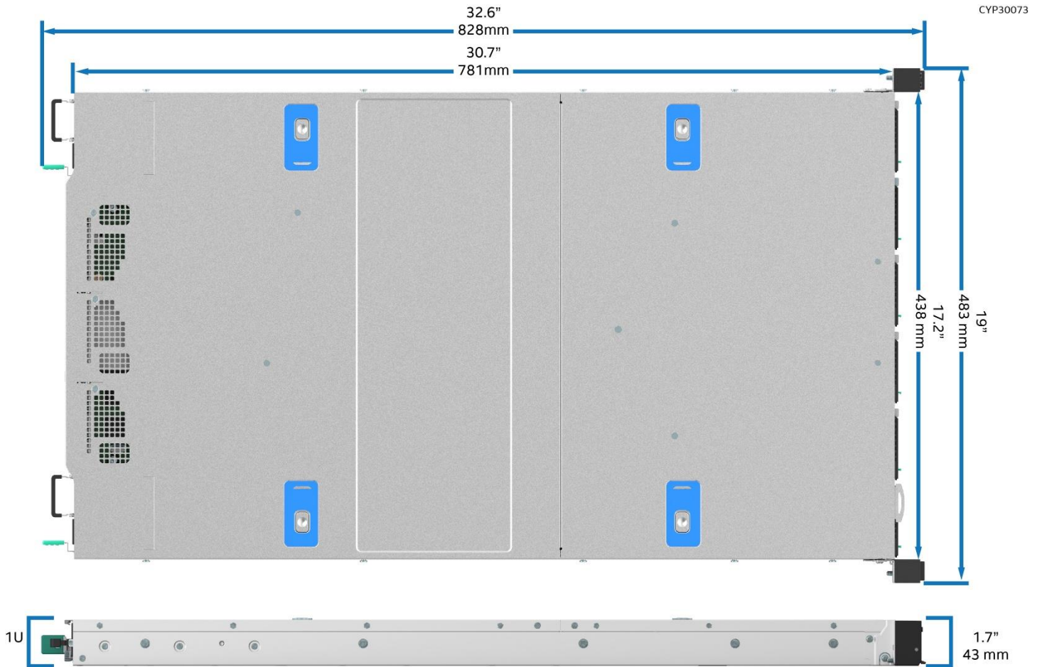
Figure 12. Chassis Dimensions
