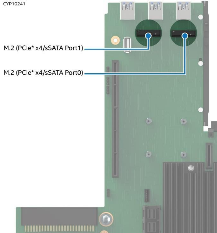
Figure 89. M.2 Module Connector Location
