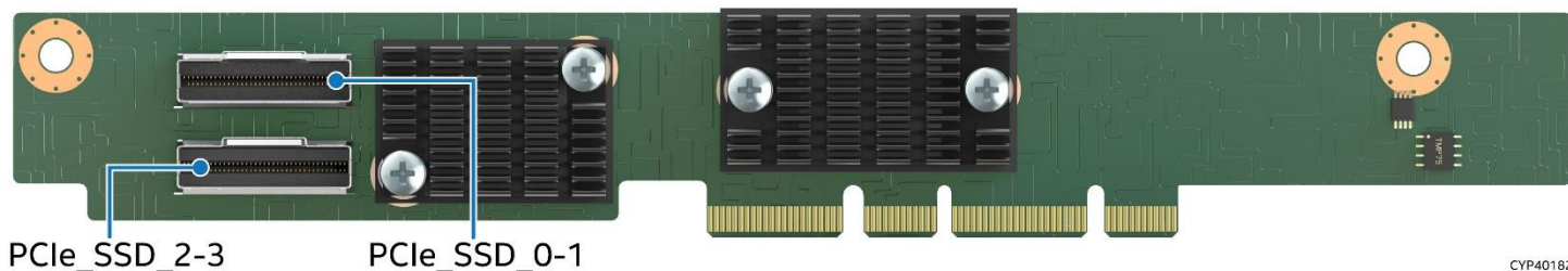
Figure 76. PCIe* NVMe* SlimSAS* Riser Card for Riser Slot #3
