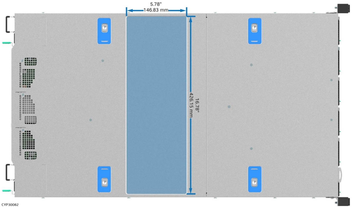
Figure 13. Label Emboss Dimensions
