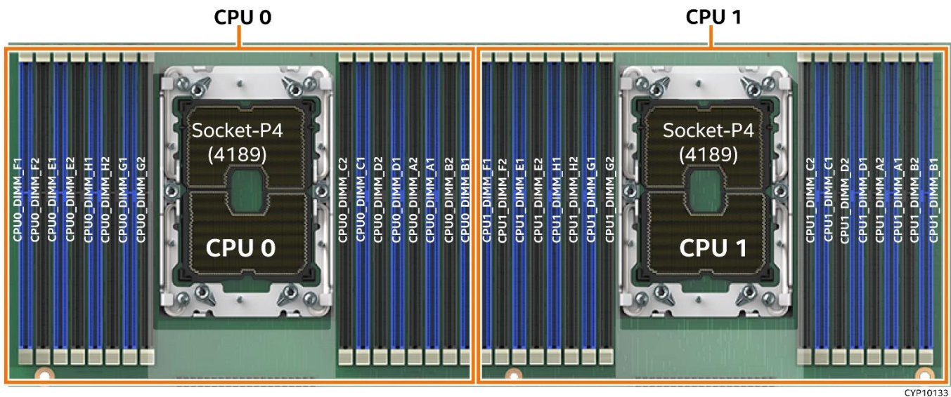
Figure 28. Intel® Server System M50CYP1UR Family Memory Slot Layout
