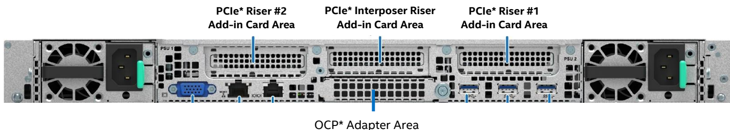
Figure 40. Server System Back Bay Add-in Card Areas
