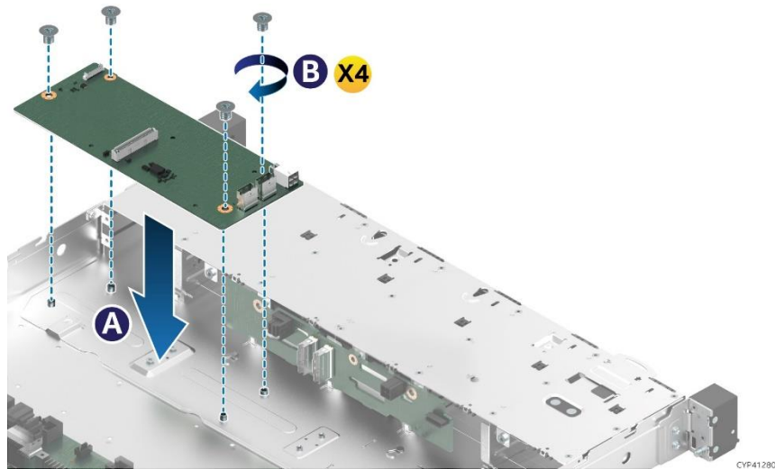
Figure 87. SAS Interposer Card Placement
