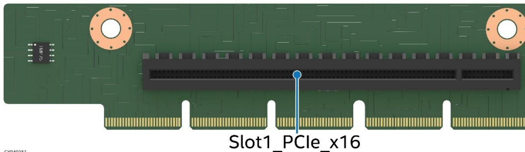
Figure 48. PCIe* Riser Card for Riser Slot #1
