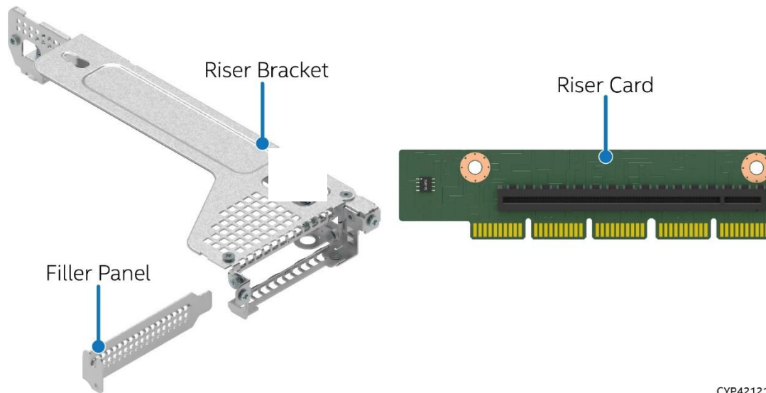
Figure 42. Riser Bracket Components
