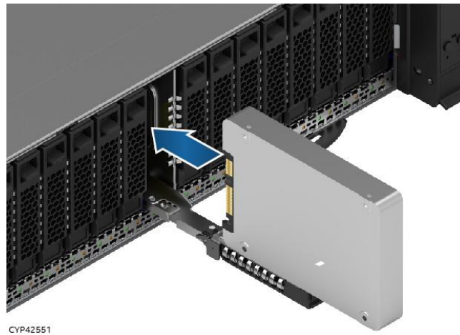
Figure 64. 15 mm Drive Insertion into 2.5" Drive Bay, Ready to Install
