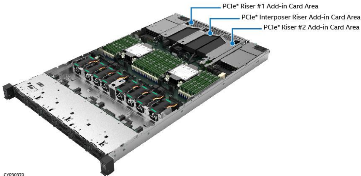
Figure 39. Server System PCIe* Riser Add-in Card Areas
