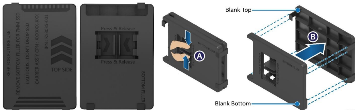
Figure 59. 2.5" Hot-Swap Drive Blank Top / Bottom and Attaching the Two
