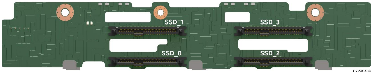
Figure 71. 4 x 2.5" SAS/SATA/NVMe* Hot Swap Backplane – Front Side
